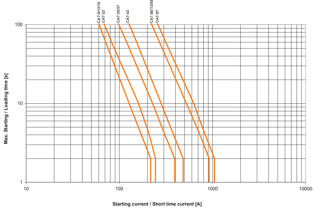
Heavy duty Starting and Regular Short-time Operation
